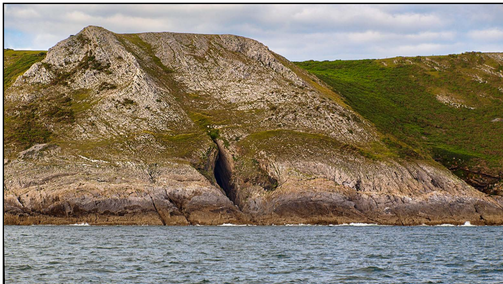
Figure 6.4.4: Minchin Hole
